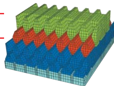
▲ 3D FLAC model of the Macrozanja showing the different levels of exploitation
